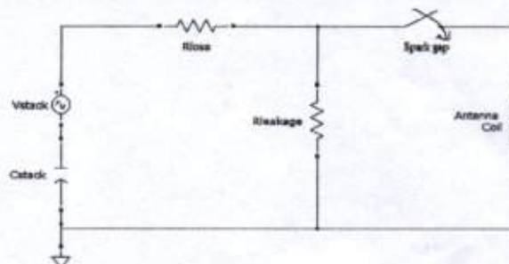
Fig. 1. Equivalent circuit of a piezoelectric device.
